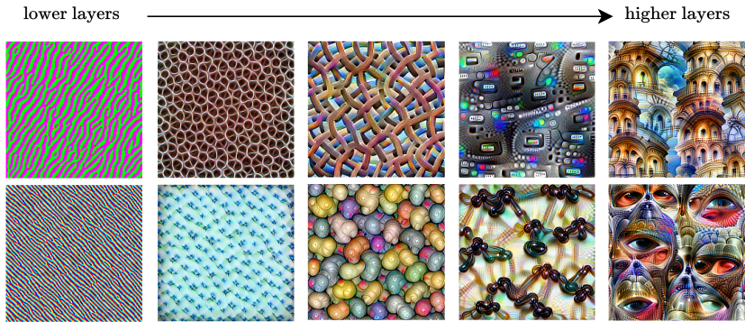
Fig. 4: Progression of data representation in the DL network ‘GoogLeNet’ [109]. GoogLeNet is an instance of a convolutional neural network (CNN), which achieves state-of-the-art performance in image analysis tasks (for an accessible introduction, see [110]). The shown images were achieved by fixing the trained model parameters and instead optimizing the pixel values of the input image in a manner that maximizes the response of certain hidden channels (in CNNs, convolutional layers usually consist of channels, which consist of units). Thus, the obtained images show what the respective channels are detecting, i.e., how the respective channels represent input images. Going from lower to higher layers, we see that channels represent edges, then textures, then patterns, then parts, then objects, such as archways and eyes. We can see that the image representations in higher layers serve to simplify classification. Detecting cars based on raw pixel values or edges, for example, is hard, but detecting cars based on channels that represent objects, such as tires, lights, and streets (and ultimately cars themselves) is much easier. These images are taken from Olah et al. [111] with permission.
