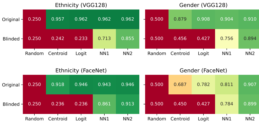
Fig. 4: “Awareness” as represented by the macro-averaged F1-scores for various classifiers, predicting sensitive features based on the face embeddings for the VGG128 model (upper panel) and the FaceNet model (lower panel). The following classifiers from scikit-learn were used: (Random) theoretical value of random guessing; (Centroid) nearest centroid classifier; (Logit) logistic regression; (NN-1,2) neural network with 1 or 2 hidden layers (100 nodes) and relu activation. A train/test split of two thirds/one third was used. The upper rows represent the scores using the original embeddings. The lower rows show the scores for the blinded embeddings. The scores are colored, ranging from red for random guessing to green for a perfect score of 1.
