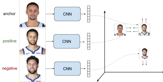
Fig. 2: General sketch of a deep FR model with triplet loss 2 . Each image is processed in the CNN model and further mapped into the embedding space such that similar faces are close together.
