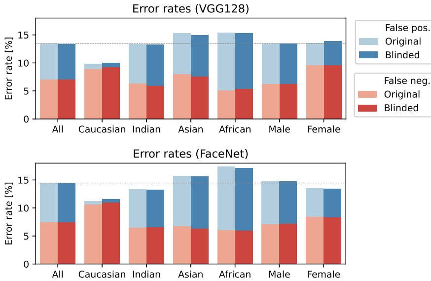
Fig. 6: Relative face recognition error rates for the VGG128 and FaceNet models. The error rates are given for all image pairs, for the different ethnic groups ( Caucasian , Indian , Asian and African ) as well as for gender ( male , female ). The horizontal line helps to indicate whether a specific group performs better or worse than the overall average. The colors distinguish the two types of errors: False positives ( blue ) are pairs of different identities which are mistakenly predicted as identical whereas false negatives ( red ) are identical faces mistakenly predicted as different. The brightness indicates the type of embedding. Light : original embeddings. Dark : blinded embedding.
