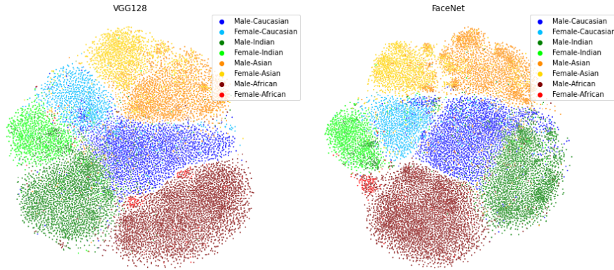
Fig. 3: t-SNE visualization (2D) of the embedding space of the RFW test set samples. The coloring is based on different labels corresponding to the sensitive features ethnicity (color) and gender (light versus dark). Left : VGG128 model. Right : FaceNet model.
