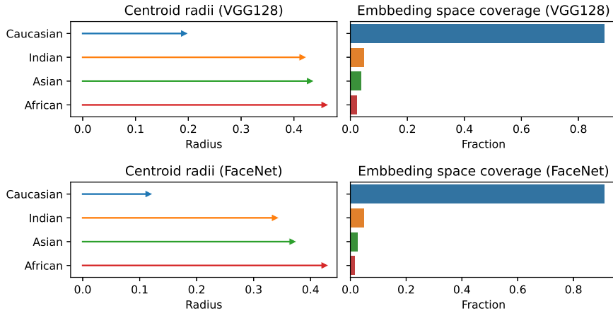
Fig. 5: Left side : Radii of the origin of the embedding space to centroids of the clusters related to ethnicity. Right side : Coverage of the embedding space associated with ethnicity. This is calculated by classifying (centroid classifier) randomly generated embedding vectors. The fractions add up to 1.
