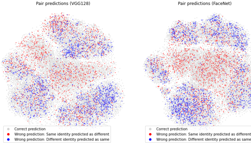
Fig. 7: This figure is derived from the t-SNE coordinates shown in Fig. 3. Each point in the plot represents the average coordinates of a pair, either positive with the same identity or negative with different identity. The grey points represent correct predictions of positive (same identity) or negative (different identity) pairs by the face recognition algorithm. Red points are the cases where positive pairs are mistakenly classified as negative pair. Blue points are the cases where negative pairs are mistakenly classified as positive pair. Left : VGG128 model. Right : FaceNet model.
